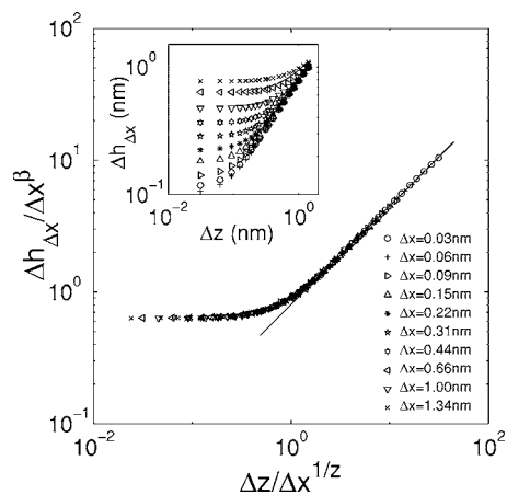
FIG. 5. Inset: 2D height-height correlation function \Delta h_{\Delta x}(\Delta z) for various angles (i.e., values of \Delta x/\Delta z ). Using the indicated scaling properties with the exponents reported in Table I, collapse of the data on a single curve is readily obtained.
