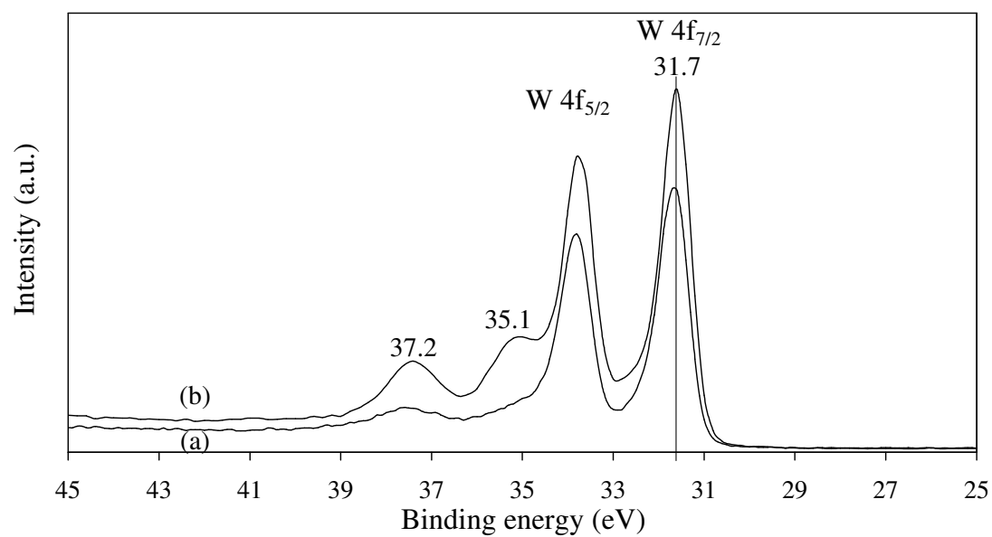
Fig. 3. W 4f XPS spectra of: (a) WC(A), (b) WC(B).
