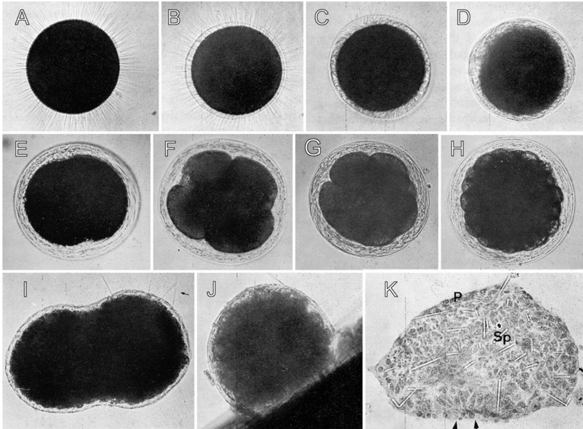
Fig. 6. Development in the tetractinomorph sponge Tetilla japonica . (A) Egg with surface filaments prior to fertilization (egg diameter 130 \mu m). (B) At fertilization a membrane is raised. (C) One minute and (D) 4 min after fertilization. (E–K) Embryo attached to the substrate. (E) Two-cell stage, 1.5 h after fertilization. (F) Four-cell stage, 3 h after fertilization. (G) Eight-cell stage, 4.5 h after fertilization. (H) Morula, 16 h after fertilization. (I) Morula formed by two fused eggs, 2 days after fertilization. (J) Side view of a 3 day old attached “larva”. (K) Longitudinal section through a 4 day old “larva”. (From Watanabe 1978, reproduced with permission of Y. Watanabe and Nat. Sci. Rep. Ochanomizu Univ., vol. 29, pp. 86, 88, and 89, © 1978 Ochanomizu University.)
