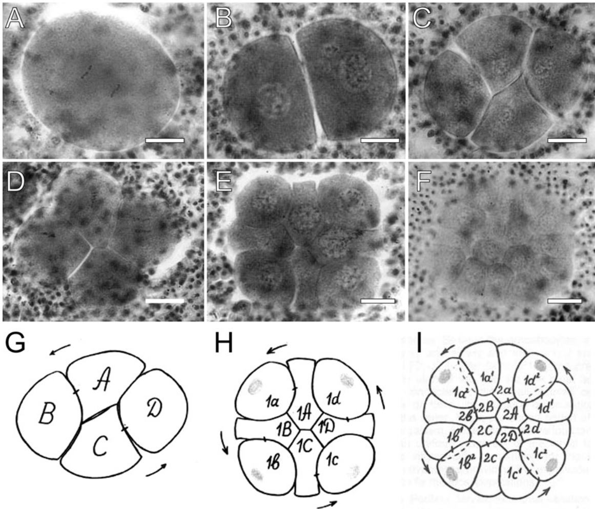
Fig. 11. Development in the homocoel (asconoid) calcarean sponge Leucosolenia complicata . (A) Anaphase of the first cleavage division. (B) Two-cell stage. (C) Second cleavage division. (D, G) Four-cell stage. (E, H) Third cleavage division. (F, I) Sixteen-cell stage. Scale bars: 2 \mu m. (From Anakina 1997, pp. 51 and 52, reproduced with permission of Berliner Geowissenschaftliche Abhandlungen, © 1997.)
