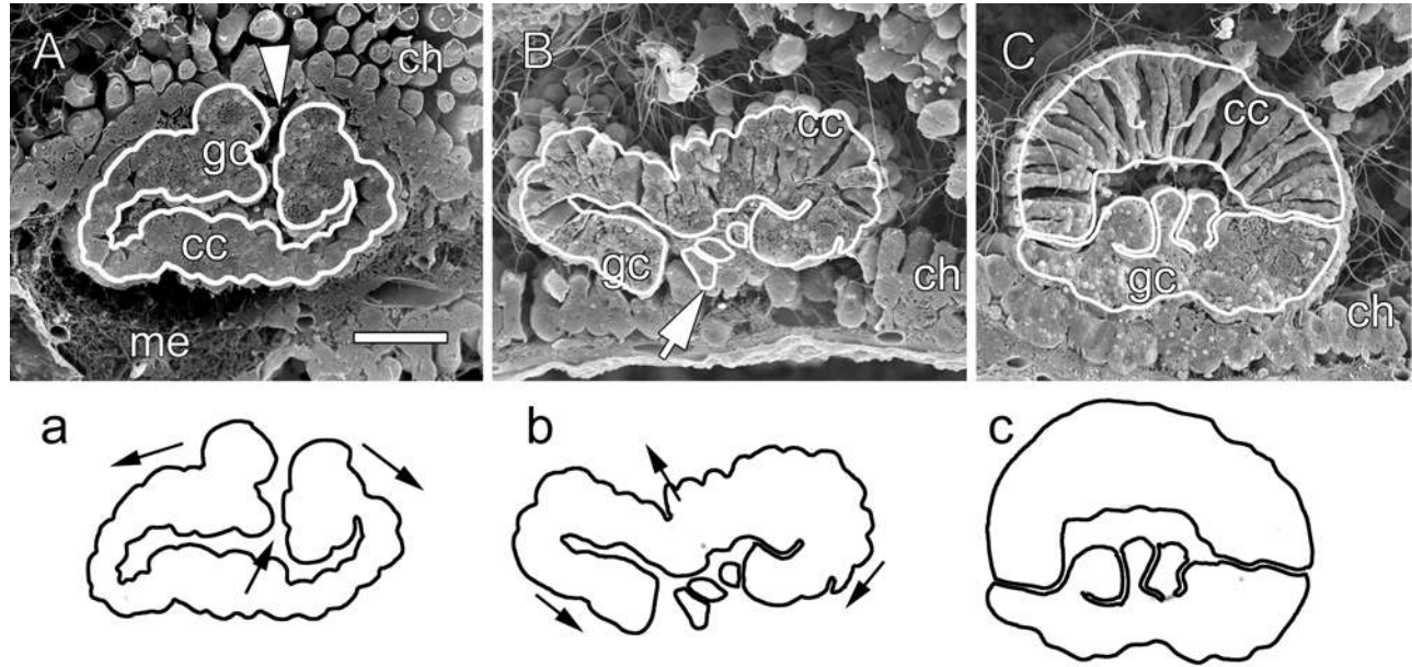
Fig. 12. SEM of the stages in inversion of the calcaronean sponge Sycon raphanus . (A, a) A stomoblastula lying in the mesohyl (me) with ciliated cells (cc) whose cilia face into the blastocoel and granular cells (gc) that form an opening (arrowhead) to the choanoderm (ch). (B, b) After inversion into the choanocyte chamber, the ciliated cells have externally facing cilia and the granular cells remain in contact with the choanoderm. Cells from the mesohyl migrate into the new larval blastocoel (arrow). (C, c) The amphiblastula larva with two distinct hemispheres of ciliated and granular cells in the choanocyte chamber. Scale bar: 10 \mu m. (S.P. Leys, unpublished data.)
