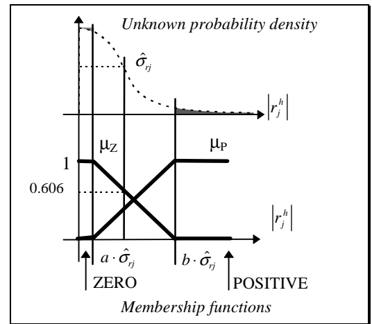
Figure 2: Residual fuzzification.
