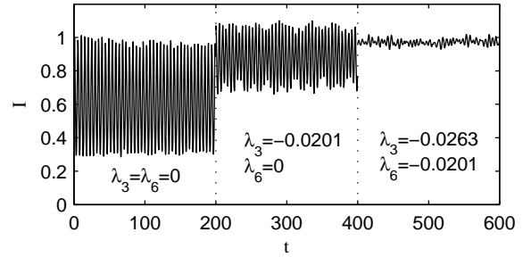
Figure 15. Intensity of the wave in the saturated regime for Hamiltonian (12) with \lambda_{k \neq 3,6} = 0 . For each value of \boldsymbol{\lambda} , the system starts with a negligible value for the intensity, and a monokinetic beam of particles.
