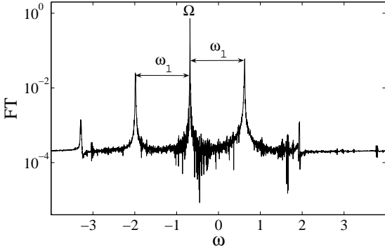
Figure 3. Fourier transform of the interaction term h(t) , as obtained from simulations of Hamiltonian (1), after saturation has been reached (same parameters in Fig. 1).
