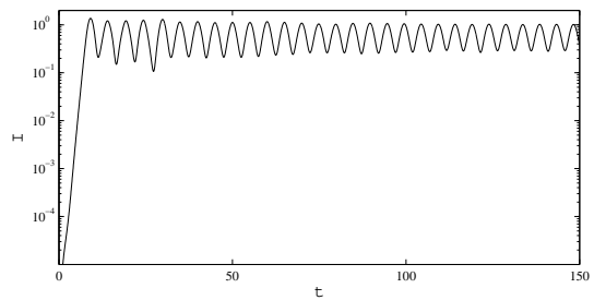
Figure 1. Normalized intensity I/N from the dynamics of Hamiltonian (1), with N = 10000 particles and H_N = 0 , P_N = 10^{-7} .
