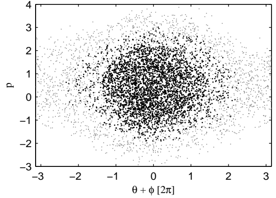
Figure 14. Snapshot of the dynamics in the (\theta, p) -plane of the N = 10000 particles at t = 1000 (the control started at t = 300 ) for Hamiltonian (12) with \lambda_3 = -0.0263 and \lambda_6 = -0.0201 . The control term is applied at t = 300 , after saturation has occurred. The grey points correspond to the particles of the chaotic sea, the dark ones form the macro-particle.
