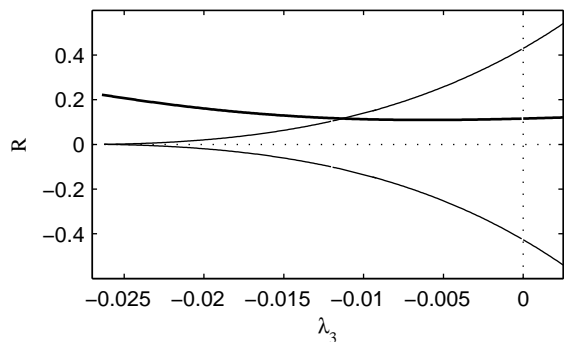
Figure 11. Residues of the elliptic (upper curve) and hyperbolic (lower curve) points with r.n. 7, and residue of the periodic point with r.n. 1 (bold curve) of Hamiltonian (11) With all the parameters set to zero except \lambda_3 .
