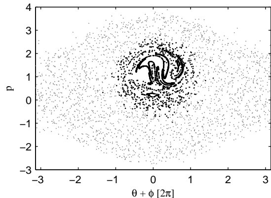
Figure 2. Snapshot of the N particles at t = 1000 , with N = 10000 (same parameters as Fig. 1). The grey points correspond to the chaotic particles, the dark ones to the particles in the macro-particle.
