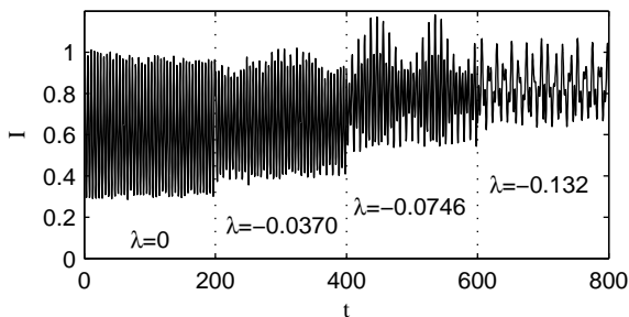
Figure 10. Intensity of the wave in the saturated regimes for Hamiltonian (8) for four values of the parameter : \lambda = 0 , -0.037 , -0.0746 and -0.1321 . For each value of \lambda , the system starts with a negligible value for the intensity, and a monokinetic beam of particles.
