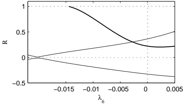
Figure 12. Residues of the elliptic (upper curve) and hyperbolic (lower curve) points with r.n. 6, and residue of the central periodic point with r.n. 1 (bold curve) for Hamiltonian (11) with \lambda_3 = \lambda_3^c and \lambda_{k \neq 3,6} = 0 as functions of \lambda_6 .
