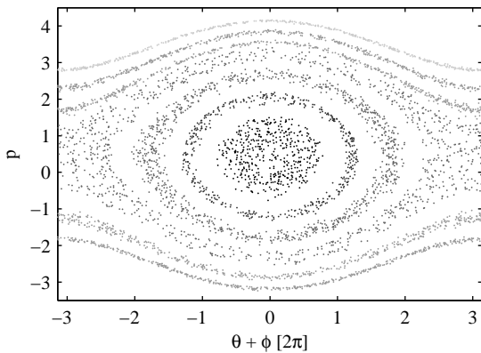
Figure 16. Poincaré section of Hamiltonian (12) with \lambda_3 = -0.0263 and \lambda_6 = -0.0201 , when the trajectory intersects the plane dI(t)/dt = 0 . The different trajectories are represented by different grey levels.
