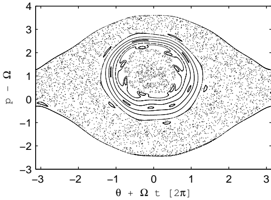
Figure 13. Poincaré section of Hamiltonian (11) with \lambda_3 = -0.0263 , \lambda_6 = -0.0201 and \lambda_{k \neq 3,6} = 0 .
