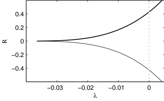
Figure 6. Residue of the elliptic (bold curve) and hyperbolic points with r.n. 7 of Hamiltonian (3).
