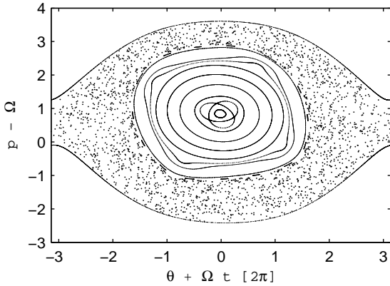
Figure 8. Poincaré section of Hamiltonian (6) with \lambda = \lambda'_c \approx -0.1321 .
