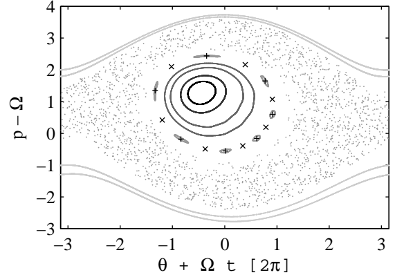
Figure 4. Poincaré section of a test-particle, described by Hamiltonian (3). The periodic orbits with r.n. 7 are marked by plus (elliptic orbit) and crosses (hyperbolic orbit).
