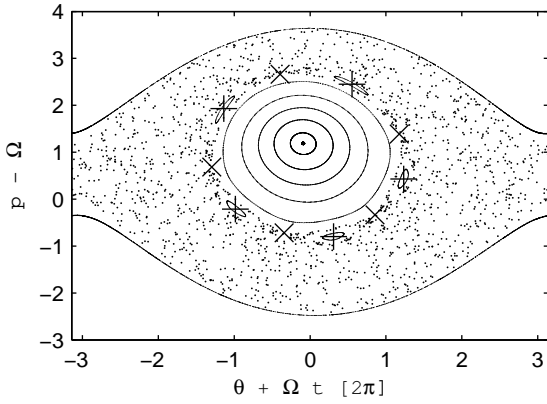
Figure 7. Poincaré section of Hamiltonian (6) with \lambda = \lambda_c \approx -0.0370 . The periodic orbits with r.n. 5 are marked by plus (elliptic orbit) and crosses (hyperbolic orbit).
