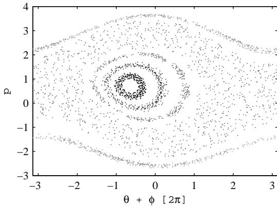
Figure 5. Poincaré section of Hamiltonian (1), when the particles intersect the plane dI(t)/dt = 0 . The different trajectories are represented by different grey levels.
