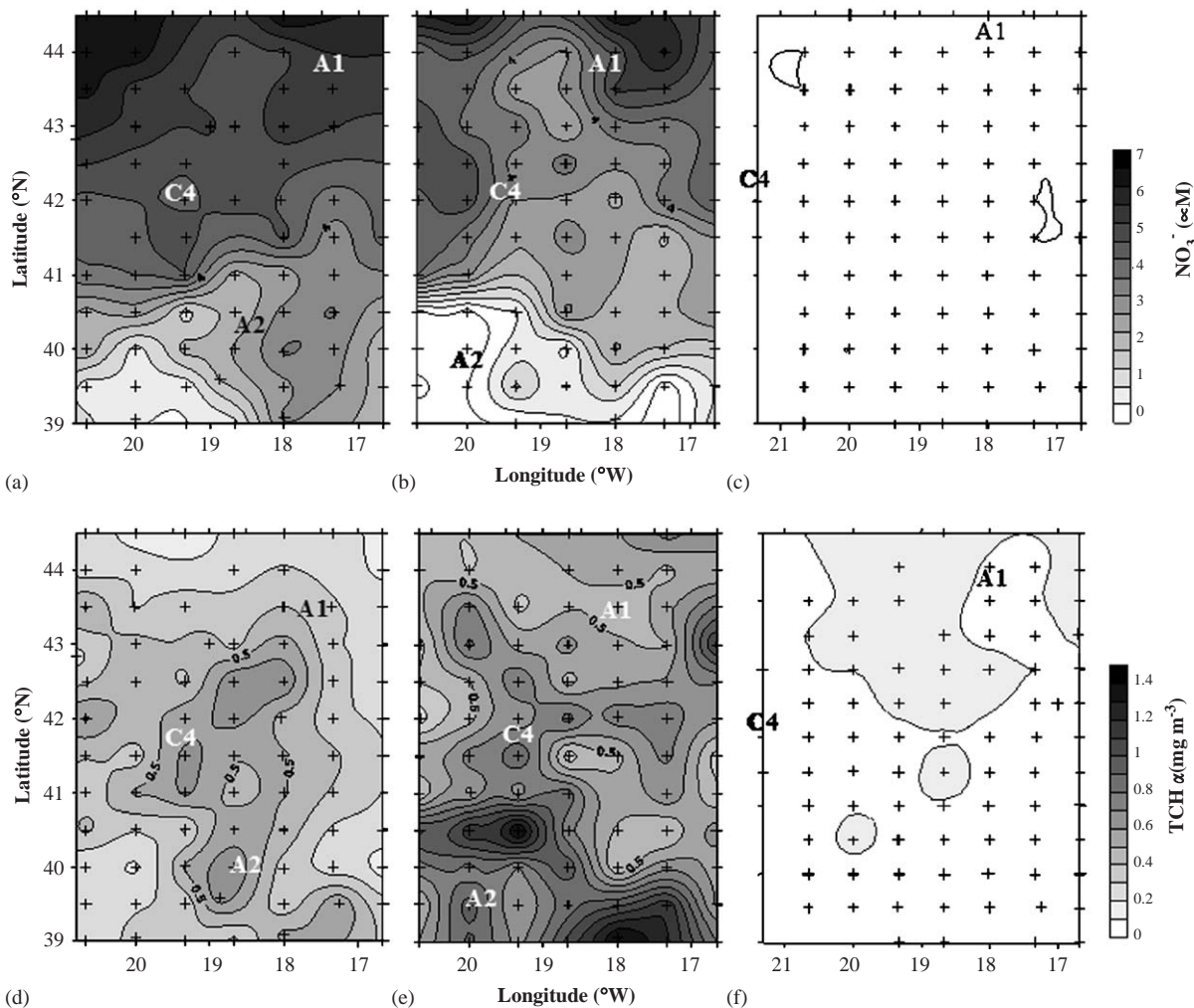
Fig. 3. Spatial distribution map of \text{NO}_3^- concentrations ( \mu\text{M} ) at 5m for: (a) winter, (b) spring and (c) late summer. Spatial distribution of total chlorophyll a concentration ( \text{mg m}^{-3} ) at 5m for: (d) winter, (e) spring and (f) late summer. A1 and A2 indicate the positions of anticyclonic eddies, and C4 indicates a cyclonic eddy.
