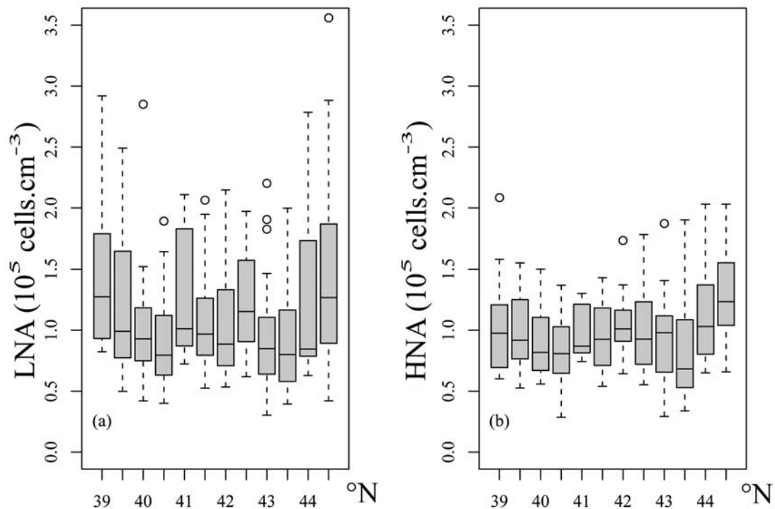
Figure 9. Box-and-whisker plots of the HNA1 and LNA abundances (10 5 cells cm -3 ) between 200 and 400 m depth as a function of the latitude.
