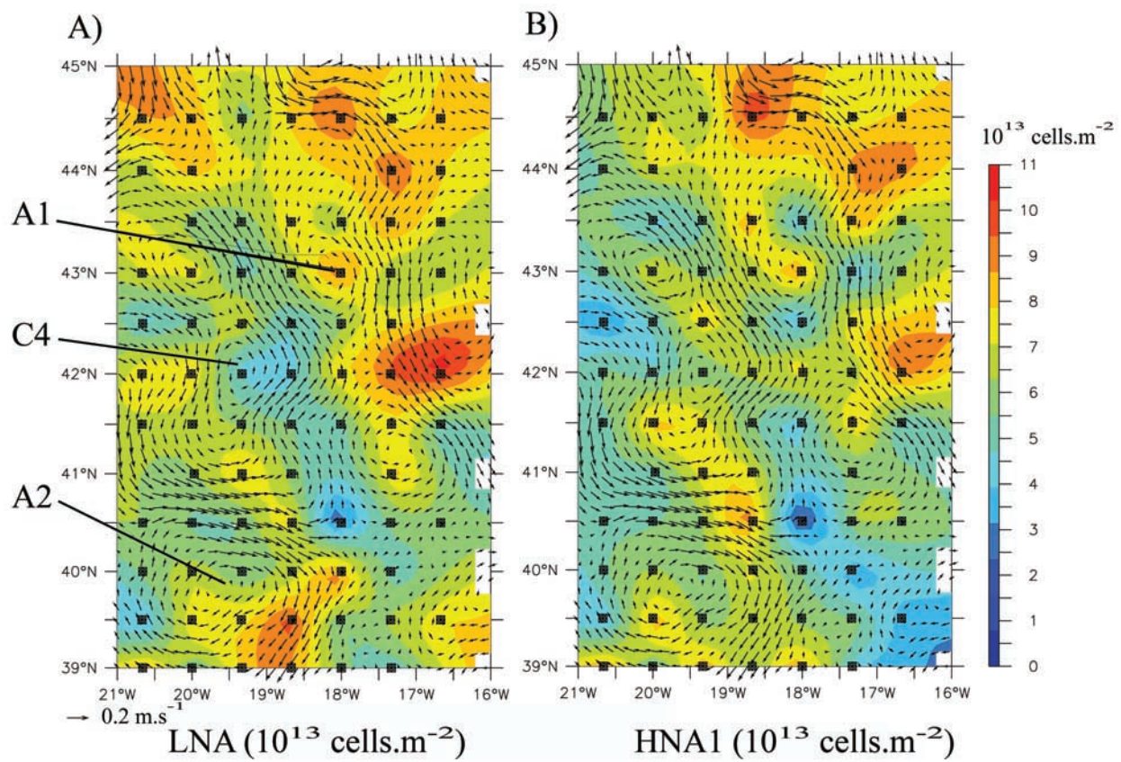
Figure 6. Upper layer geostrophic current field superimposed on the bacteria abundances integrated between 0 and 300 m depth. (a) LNA integrated values (10 13 cells m -2 ). (b) HNA1 integrated values (10 13 cells m -2 ). Labeled mesoscale features: A1 and A2, anticyclonic gyre; C4, cyclonic gyre.
