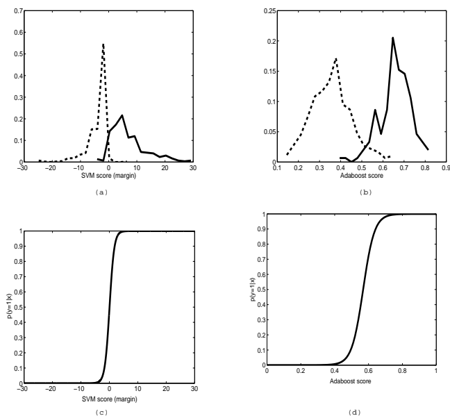
Fig. 4. Example of calibrated probabilities produced with Platt scaling method for SVM classifier and Adaboost classifier on the pedestrian data set. (a) and (b) are The histograms for p(\mathbf{x}|y = \pm 1) . The solid line is p(\mathbf{x}|y = 1) , while the dashed line is p(\mathbf{x}|y = -1) . (c) and (d) are the posterior probability distributions, defined by a sigmoid function fitting from a training set.
