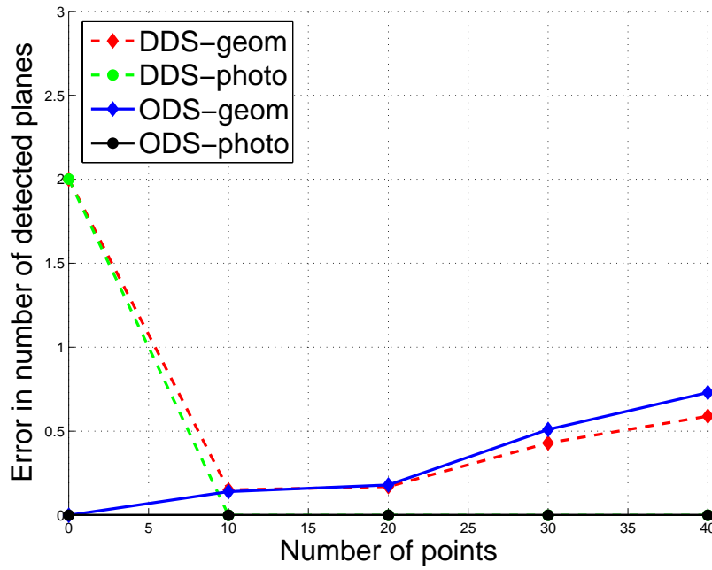
Figure 6: Comparison of the error in the number of detected planes for varying number of points.
