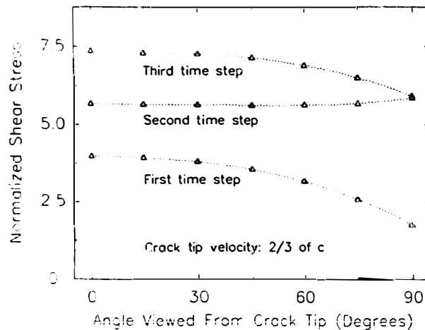
Fig. 12. Shear stress development around the “running” crack tip, from the time step to time step after a crack tip jump. The ratio \sigma_{\theta 3}(\theta) / \sigma_{\theta 3}(0) does not develop smoothly.
