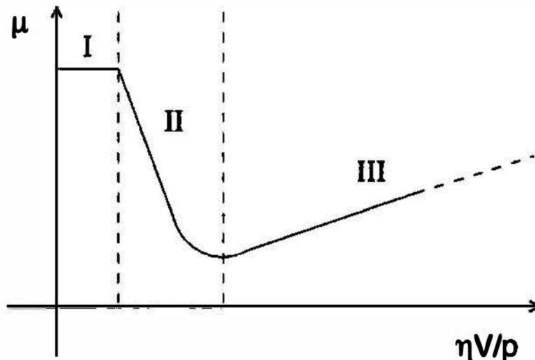
FIG. 1. Stribeck's curve.
