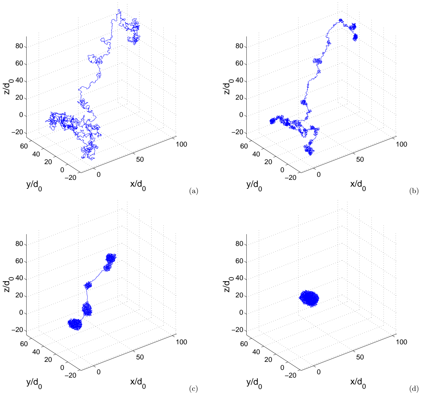
FIG. 1: Molecular dynamics simulation of a N = 3000 homopolymer. (a) A self-avoiding random walk generated by a Monte-Carlo method ( t = 0 ). (b) Nucleation centers appear ( t = 3 \cdot 10^4 \Delta t ), this state is characterized by a set of pearls separated by stretched chains. (c) Merging of pearls accompanied by a shrinking of the polymer size ( t = 3 \cdot 10^5 \Delta t ). (d) Globular state ( t = 6 \cdot 10^5 \Delta t ).
