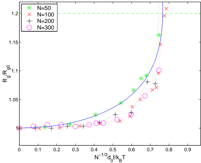
FIG. 4: Mean gyration radius R_g/R_{g0} as a function of the normalized tension N^{-1/3}f/k_B T , for various values of N . The solid line is the theoretical result from equation (6) (with \beta = 1.7 ); the horizontal dashed line represent the critical radius R_A/R_e = (7/4)^{1/3} , and the vertical one is the critical normalized force f_A^* .
