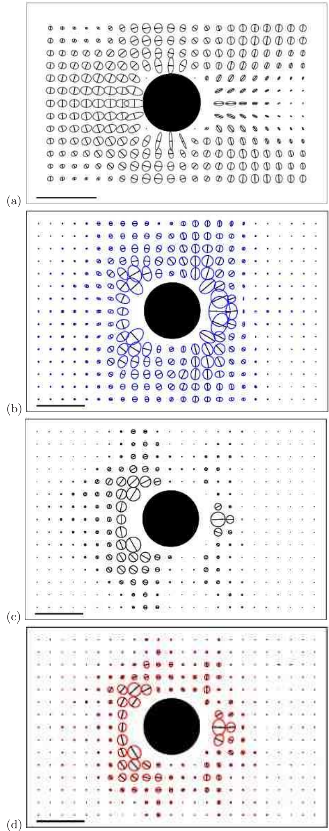
Fig. 8. Wet foam flowing around an obstacle (Fig. 1a). Measurements of \bar{U} (a) and \bar{V} (b) yield, through eq. (7) with quadratic plasticity function h , the theoretical prediction of \bar{P} (c), in good agreement with its measurement (d). Scale: for \bar{U} , bar= 1 (no unit); for \bar{V} and \bar{P} : bar= 1 s^{-1} .
