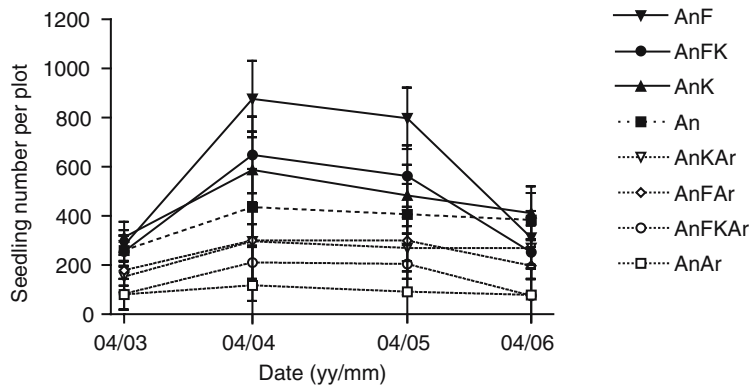
Figure 4. Mean numbers \pm SE of Anthyllis vulneraria seedlings per plot recorded during the last four months of the experiment in plots where this species was initially present. Continuous lines represent plots with the two grasses, Festuca arvernensis and Koeleria vallesiana , dotted lines the plots with grasses and Armeria arenaria individuals, and the thick dotted lines the plots with initial monocultures of Anthyllis vulneraria . An: Anthyllis vulneraria ; Ar: Armeria arenaria ; F: Festuca arvernensis ; K: Koeleria vallesiana .
