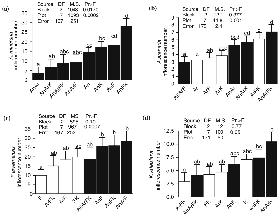
Figure 3. ANOVAs and mean numbers \pm SE of inflorescences for (a) Anthyllis , (b) Armeria , (c) Festuca and (d) Koeleria individuals in the different plots containing these species, recorded at the first flowering peak (June 2003). For each species means with the same letters do not differ significantly at the 5% level with a Tukey test. An: Anthyllis vulneraria ; Ar: Armeria arenaria ; F: Festuca arvernensis ; K: Koeleria vallesiana .
