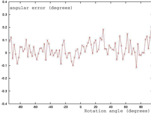
Figure 3: Angular error
