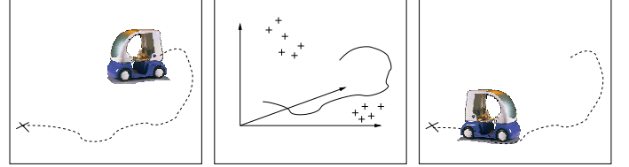
Fig. 4. Principle of vision based localization. 1) vehicle freely moves and records a video sequence. 2) trajectory and visual features of the video are reconstructed. 3) vehicle can localize itself and take the same path.
