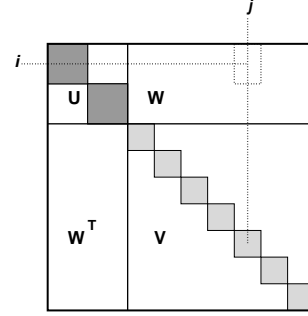
Fig. 3. Structure of J^T J matrix
