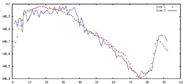
Figure 4. Registration with GPS reference, top: in horizontal plane, bottom: on altitude axis. Continuous line represents GPS trajectory and points represent estimated key positions. Coordinates are expressed in meters .
