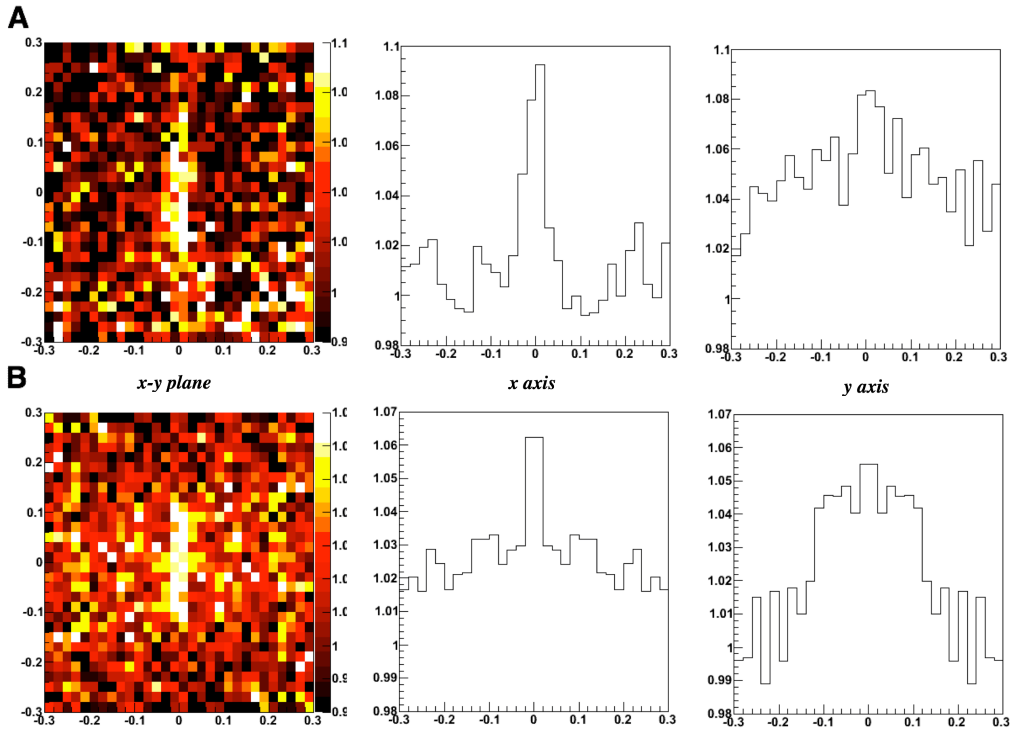
FIGURE 3. Atom correlation signals: (A), for opposite momenta, (B), for colinear momenta. The left image shows the signal in the x - y plane. The next two in each row show the signals along one axis and integrated along the other. The second line (B) is simply a manifestation of the Hanbury Brown Twiss effect. In both cases the correlation function is anisotropic because of the initial anisotropy of the source. The normalization is such that unity corresponds to no correlation.
