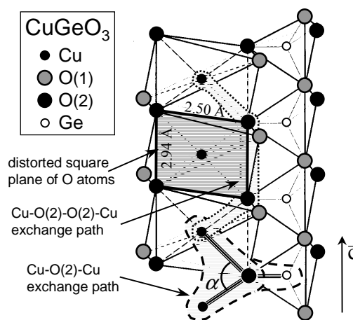
Fig. 1. Schematic structure of \text{CuGeO}_3
