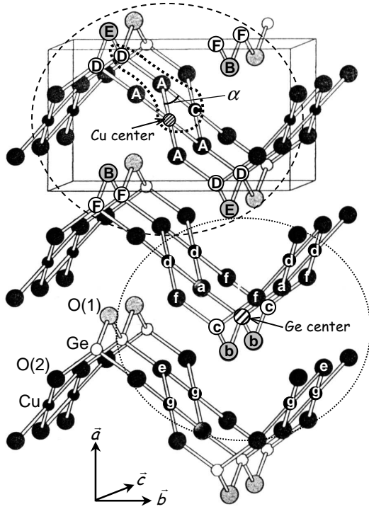
Fig. 4. Structure of CuGeO 3 . The Cu and Ge environments are materialized: starting from the dashed Cu and Ge absorbers, the atoms labelled "A", "B", ... "F" (for Cu) and "a", "b", ... "g" (for Ge) are their neighbors going from the closest to the furthest ones that were accessible in the EXAFS experiment.
