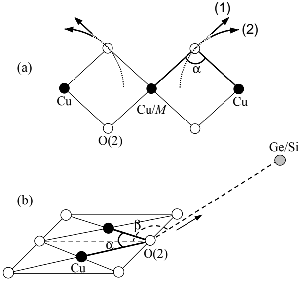
Fig. 9. Schematic view of the local deformation, due to M/Cu (a) and Si/Ge (b) substitution, assumed for the calculation of the local Cu (or M )- O(2) - Cu angle \alpha (see text for the different scenarii).
