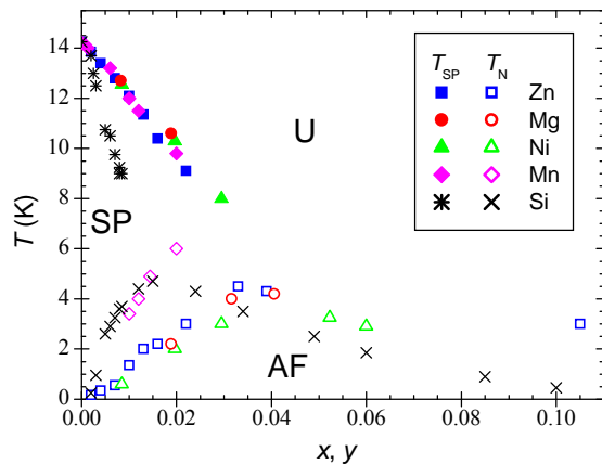
Fig. 2. (Temperature - concentration) magnetic phase diagram for CuGe 1-x Si x O 3 and Cu 1-y M y GeO 3 , with M = \text{Zn, Mg, Ni, and Mn} .
