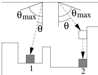
Figure 1: Discrete model. SOS shadowed ballistic deposition process. Particle 2 hits a column side, then falls down.
