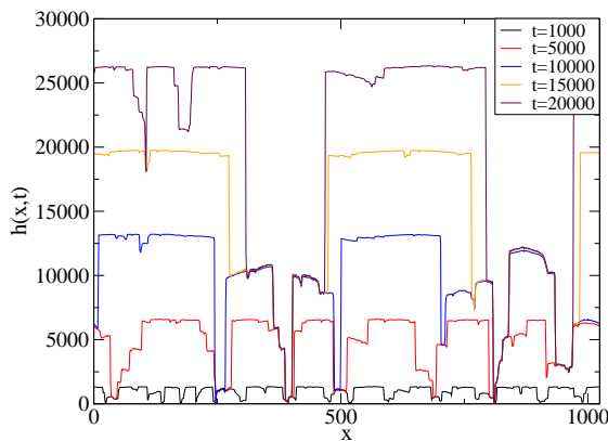
Figure 2: Discrete model. Interface h(x,t) at time t = 1\,000 , 5\,000 , 10\,000 , 15\,000 and 20\,000 for \theta_{max} = 60^\circ and L = 1024 .
