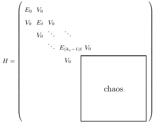
FIG. 7: Sketch of the effective Hamiltonian matrix that describes the coupling between the regular island and the chaotic domain for one particular symmetry class (i.e., for “even” or “odd” states with respect to time-reversal symmetry). The regular part (upper left band) includes only components that are coupled to the island’s central state by the s/l resonance. In the simplest possible approximation, the chaotic part consists of a full sub-block with equally strong couplings between all basis states with actions beyond the outermost invariant torus of the island.
