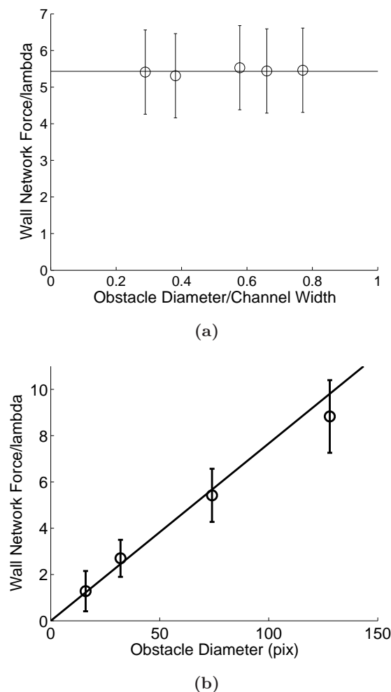
FIG. 5: Network contribution to the yield drag F_Y^n (expressed in unit of \lambda ), measured in Potts model simulations with A = 100 \text{ pix}^2 ( \Phi = 0.005 ). (a) F_Y^n versus w_c , for d_0 = 74 \text{ pix} ; the solid line is the average (value 5.43). (b) F_Y^n versus d_0 , for w_c = 256 \text{ pix} ; the solid line is a linear fit with zero intercept, F_Y^n = 0.77 d_0/\sqrt{A} .
