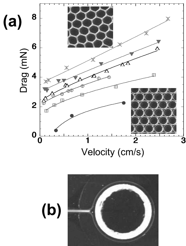
FIG. 9: (a) Drag versus velocity for various distances h between the top plate and the bottom solution: 2.0 ( \bullet ), 2.5 ( \square ), 3.0 ( \circ ), 3.5 ( \triangle ), 4.0 ( \blacktriangledown ) and 4.5 mm ( \times ). Here A = 16.0 \text{ mm}^2 and d_0 = 3 \text{ cm} . The curves are the best fits by the formula F = F_Y^t + A \times V^a . Snapshots of the foam of the smallest (bottom) and highest (top) h are also displayed. (b) Photograph of a single soap film pulling on the left side of the circular obstacle.
