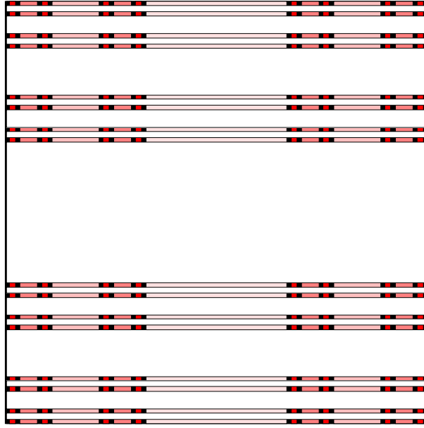
FIGURE 3. Various components \Gamma_+^{(n)} of the forward trapped set for the open baker B_{r_{sym}} . Various red/grey scales (from light to dark) correspond to n = 1, 2, 3, 4 .
