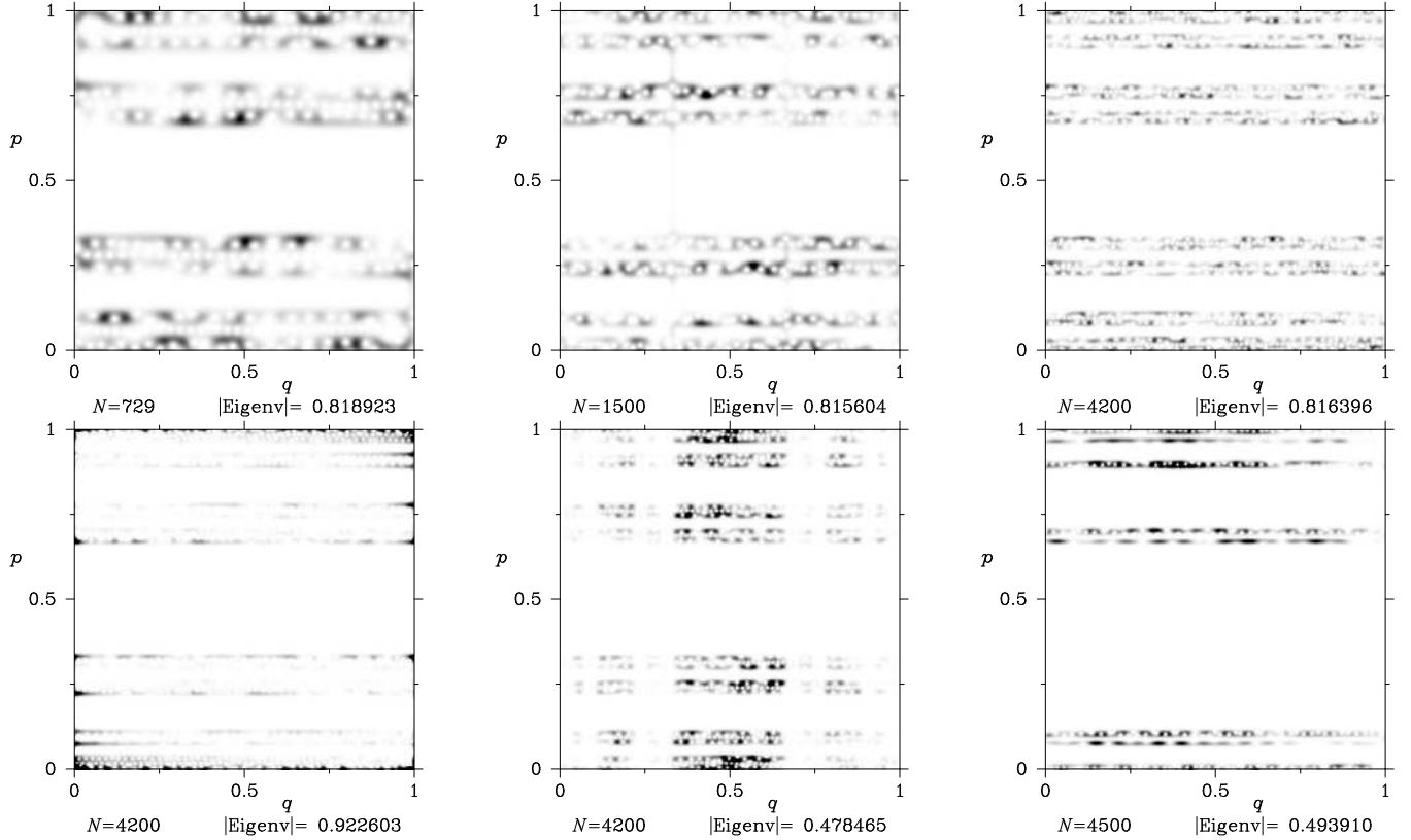
FIGURE 7. Husimi densities of (right) eigenstates of B_{r,N} (black=large values, white=0). Top: 3 eigenstates of B_{r_{sym},N} with |\lambda_N| \approx \sqrt{\Lambda_{nat}} . Bottom left, center: two eigenstates of B_{r_{sym},N} with different |\lambda_N| . Bottom right: one eigenstate of B_{r_2,N} .
