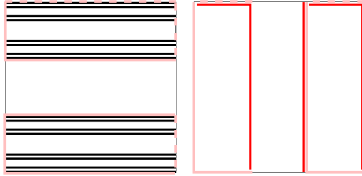
FIGURE 4. On the left, we show the backward trapped set \Gamma_+ for the symmetric open baker B_{\mathbf{r}_{sym}} (black), and the discontinuity set D(B_{\mathbf{r}_{sym}}^{-1}) (pink/light gray). Their union gives \Gamma_+ \sqcup D_{-\infty} , which contains the support of semiclassical measures (see Thm. 1, i ). The dotted lines indicate identical points on \mathbb{T}^2 . On the right, we show the backwards image B_{\mathbf{r}_{sym}}^{-1}(D(B_{\mathbf{r}_{sym}}^{-1})) involved in Thm 1, iii ) (pink/light gray), and the projection on \mathbb{T}^2 of the set \Sigma \setminus \Sigma'' defined in (2.10) (red/dark gray).
