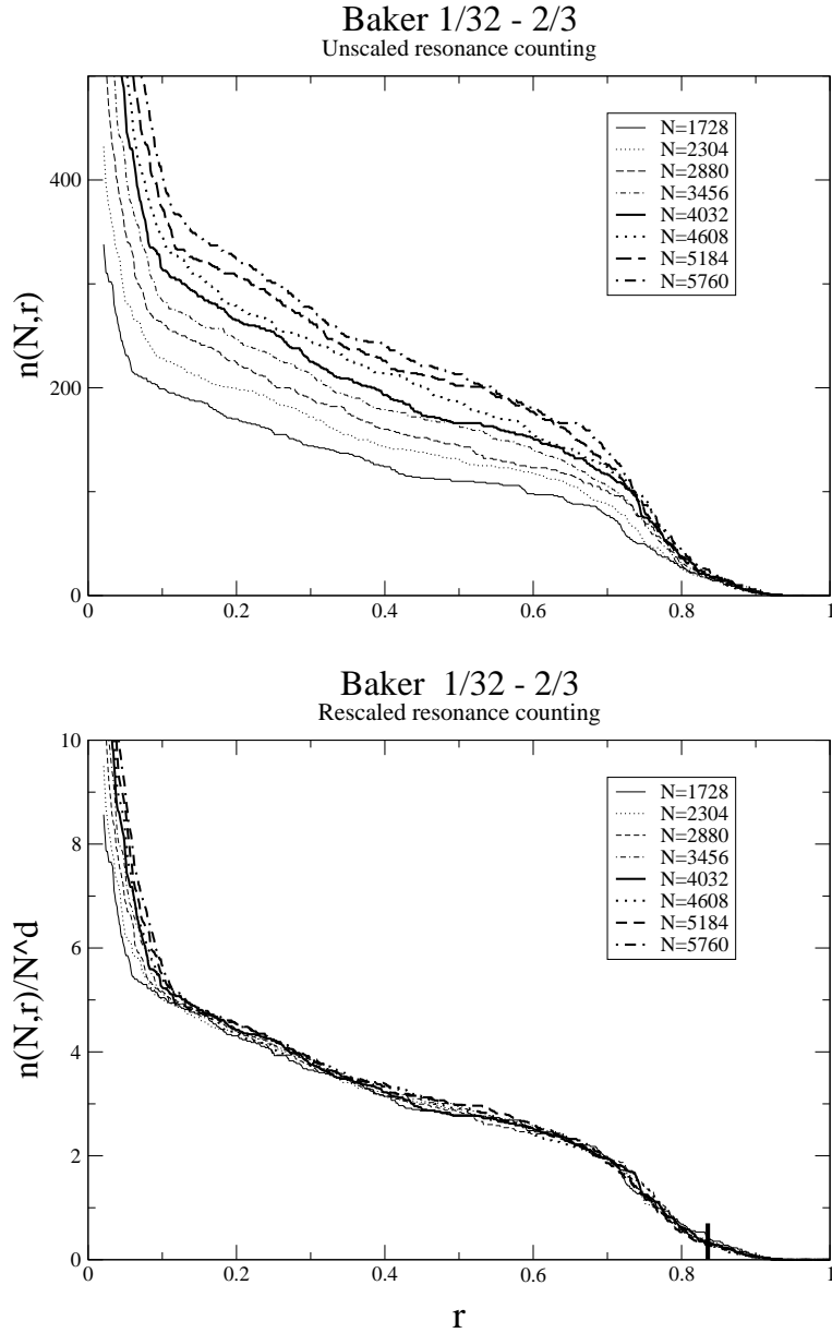
FIGURE 6. Top: spectral counting function for the asymmetric baker B_{\mathbf{r}_{asym}} , for various values of Planck's constant N . Bottom: same curves vertically rescaled by N^{-d_0} . The thick tick mark indicates the radius \sqrt{\Lambda_{nat}} corresponding to the natural measure.
