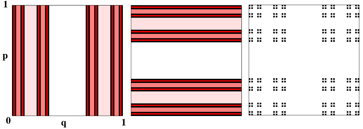
FIGURE 2. In black we approximate the forward (left), backward (center) and joint (right) trapped sets for the symmetric open baker B_{r_{sym}} . On the left (resp. centre), red/gray scales (from white to dark) correspond to points escaping at successive times in the future (resp. past), that is to sets M_n (resp. M_{-n} ), for n = 1, 2, 3, 4 .
