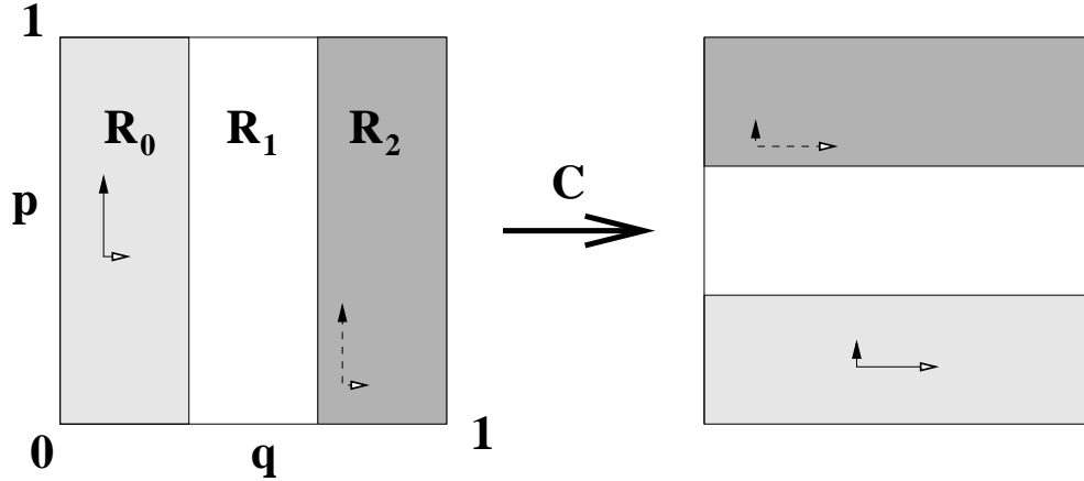
FIGURE 1. Sketch of the closed baker's map \hat{B}_{\mathbf{r}} , and its open counterpart B_{\mathbf{r}} , for the case \mathbf{r} = \mathbf{r}_{sym} = (1/3, 1/3, 1/3) . The three rectangles form a Markov partition.
