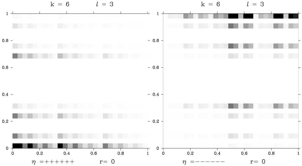
FIGURE 9. Walsh-Husimi densities for the extremal eigenstates \psi_{+,N} , \psi_{-,N} of \tilde{B}_N , with N = 3^6 , \ell = 3 . These are coarse-grained versions of the Bernoulli measures \mu_{\mathbf{P}_+} and \mu_{\mathbf{P}_-} .
