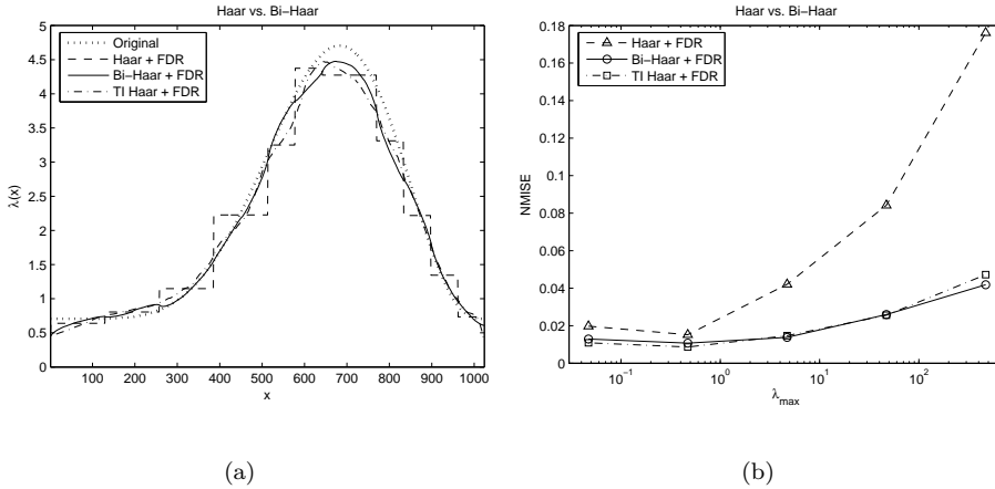
Fig. 1. Denoising the “Smooth” function (length = 1024). Estimates from Haar, Bi-Haar and TI Haar (undecimated) are compared. FDR is set to 0.05 and J = 7 . (a) denoising results; (b) NMISEs.
