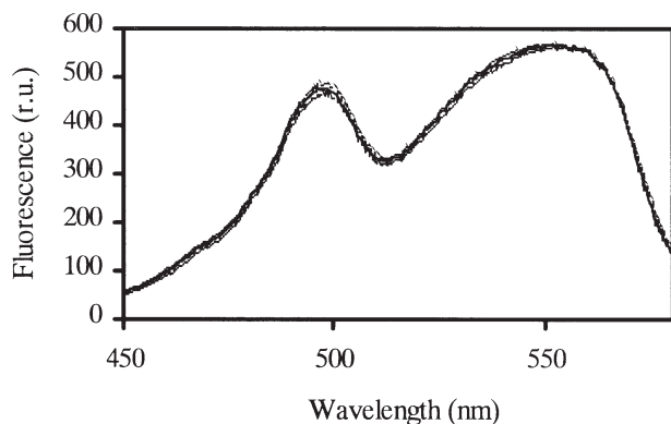
Fig. 6. Diurnal variations of the HITACHI-corrected fluorescence excitation of T. thiebautii phycocyanin in surface waters (solution in phosphate buffer 0.1 mol L -1 pH = 6.5). Mean, mean–standard deviation and mean + standard deviation curves determined from five spectra recorded each 3 h between dawn and dusk (from 6:00 to 18:00 h). The coefficient of variation was lower than 3% beyond 479 nm and between 3% and 6% from 450 to 479 nm.
