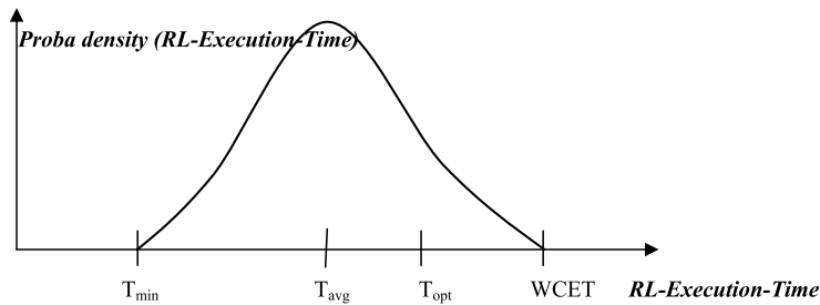
Fig. 8. RL-Execution-Time distribution
