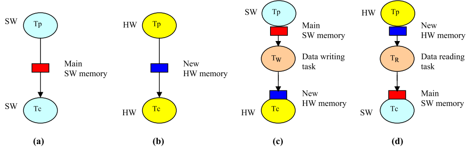
Fig. 3. Memory and Tasks implementations for HW/SW communications
