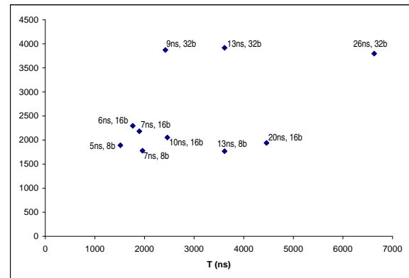
Figure 4: Bitwidth and clock period exploration
