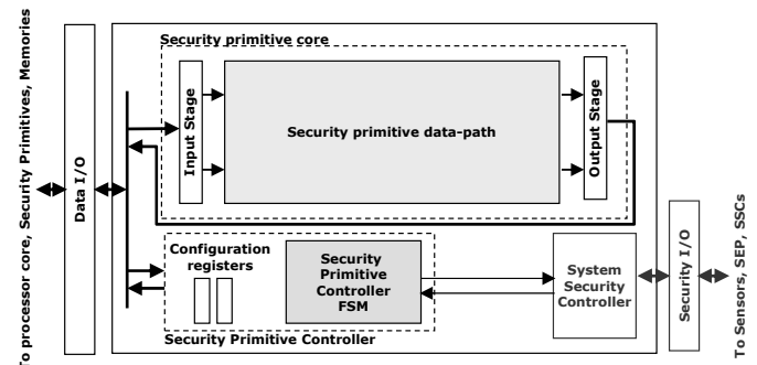
Fig. 2. The security primitive architecture. The Security Primitive Controller manages the flexibility of the primitive and the Security System Controller deals with the detection of abnormal activity using specific sensors
