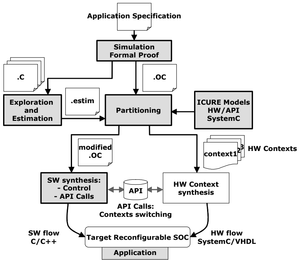
Fig.3 - EPICURE global design Flow
