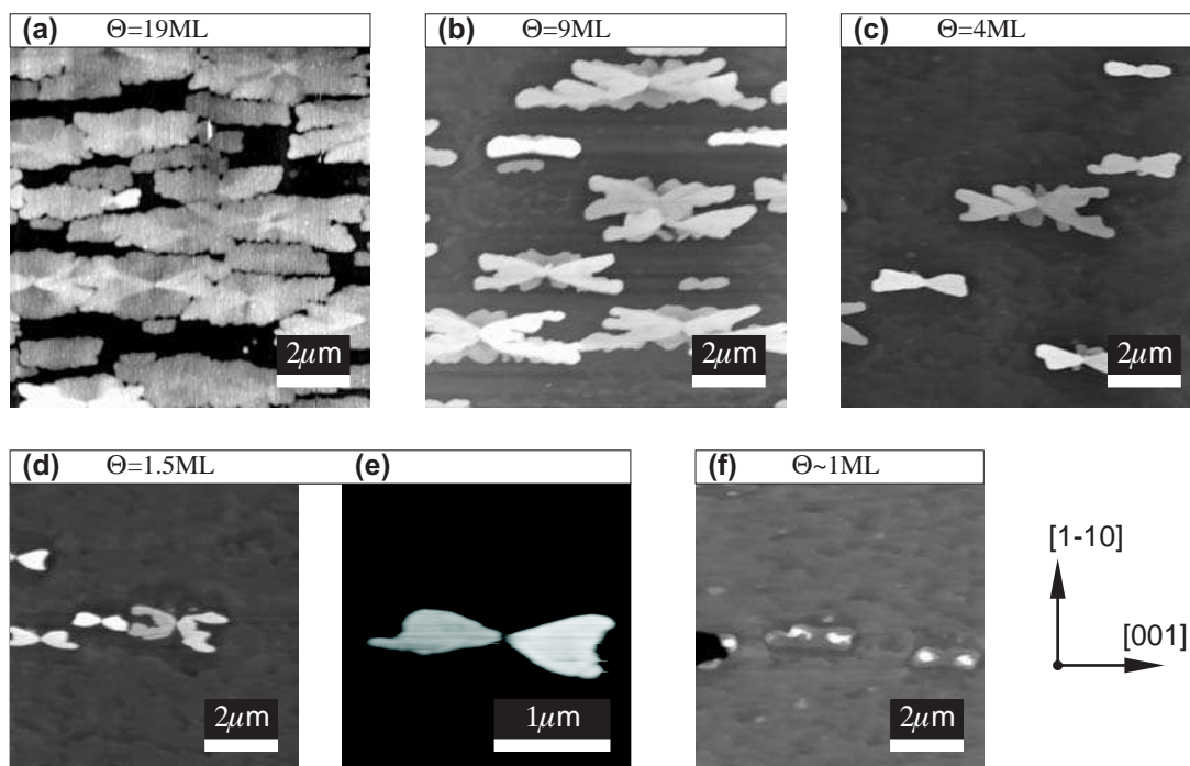
Figure 24. ex situ AFM images of Fe grown at 800\text{ }^\circ\text{C} on \text{W}/\text{Mo}_{10}\text{W}_{90}(110) . Notice the different scale in (e).
