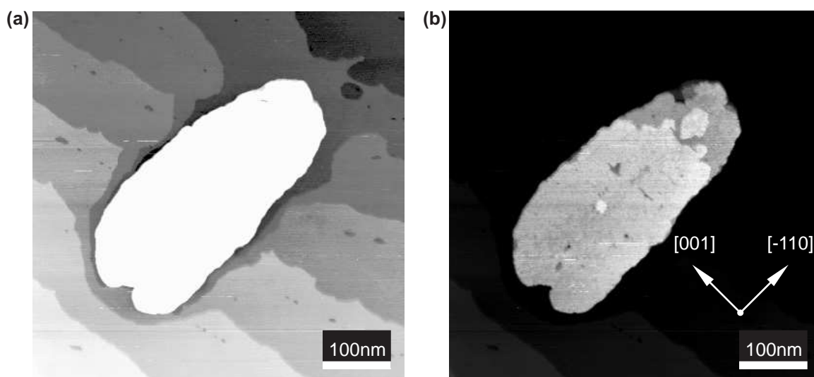
Figure 25. STM image revealing the etching process around wedge-shaped flat Fe islands grown on \text{Mo}(110) at 525\text{ }^\circ\text{C} . A different color scale is used in (a) and (b), to highlight the steps of the buffer layer and the top of the dot, respectively
