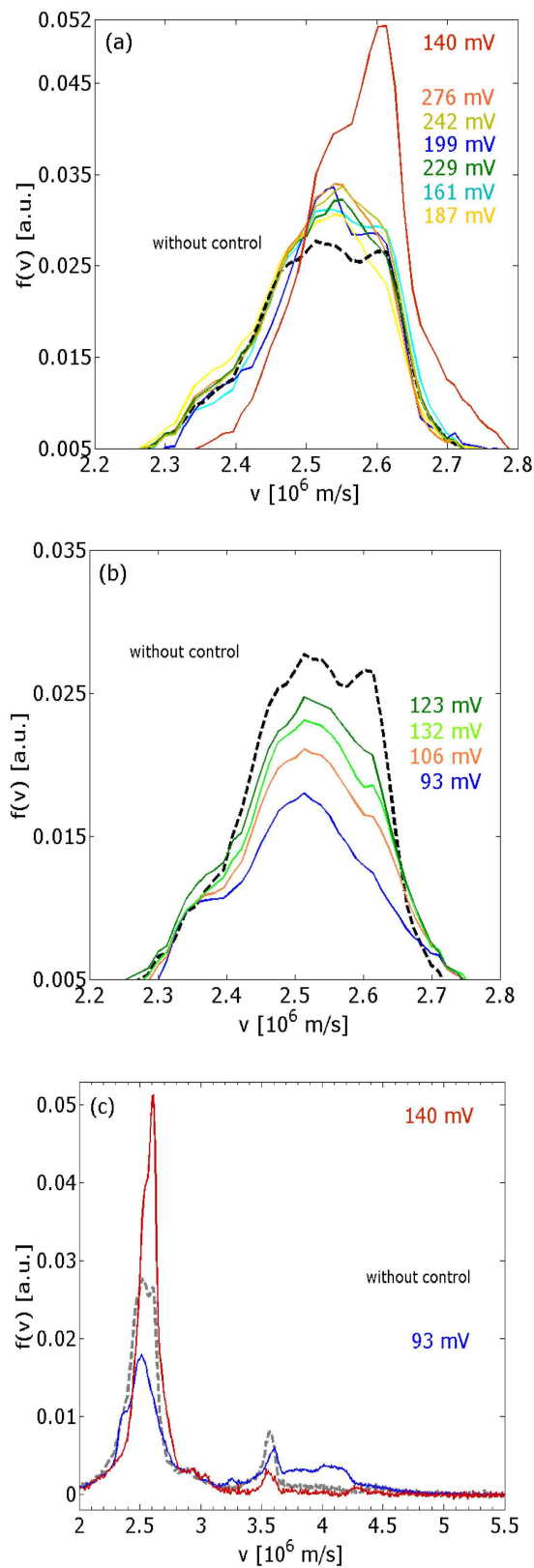
FIG. 16: Enlargement of velocity distribution functions close to initial beam velocity for different control amplitudes: (a) larger, (b) lower than experimentally optimized amplitude 140 mV. (c) velocity distribution functions for three different control amplitudes at fixed control phase equal to 0^\circ . The overlap parameter is s = 1.27 .
