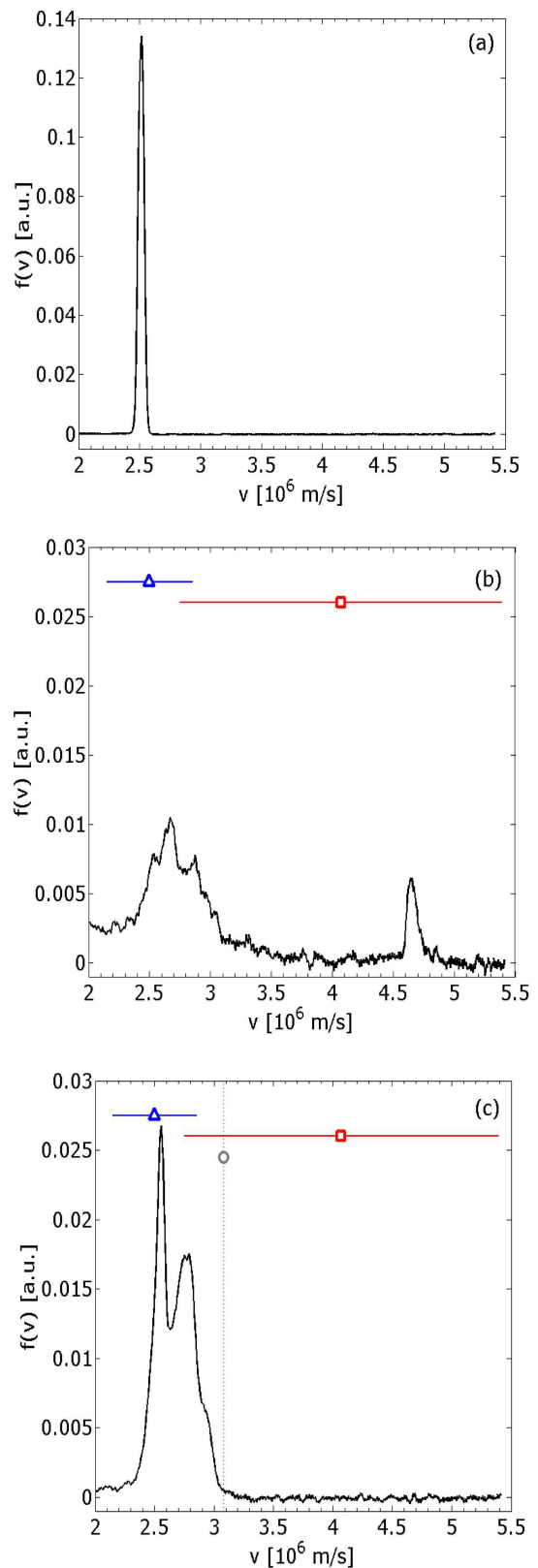
FIG. 9: Beam velocity distribution functions at the output of the TWT for s = 0.85 : (a) test beam ( I_b = 50 nA) without electrostatic wave, (b) with helix mode (trapping domain shown by red line with phase velocity marked by a square) and beam mode (trapping domain shown by blue line with phase velocity marked by a triangle) at 30 MHz, (c) with an additional controlling wave at 60 MHz and phase velocity given by grey circle and dotted line.
