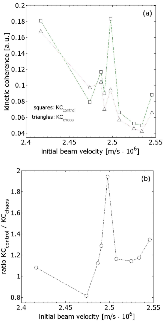
FIG. 17: Kinetic coherence versus initial beam velocity with optimized control term amplitude (140 mV) and phase ( 0^\circ ). (a), squares (resp. triangles) show the values for velocity distribution function obtained with (resp. without) applied control term. (b), Ratio between kinetic coherence measured with and without control for different initial beam velocity. The overlap parameter is s = 1.27 .
