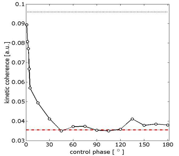
FIG. 6: Kinetic coherence versus the phase introduced in the approximate control term given by Eq. (17). The red dash-dotted line indicates the kinetic coherence value for the non-controlled case and the dotted line the kinetic coherence value for the approximate control term. The overlap parameter is s = 1.27 .
