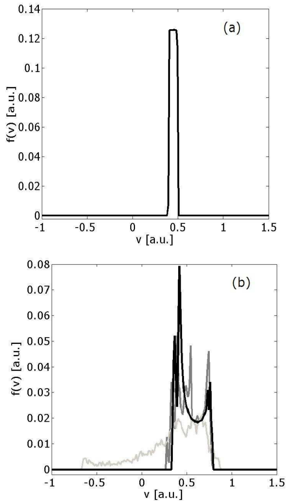
FIG. 4: (a): initial beam velocity distribution function for s = 0.85 . (b): final beam velocity distribution function without control term (9) (light gray line), with the exact control term (black line) and with the approximate control term (16) (dark gray line).
