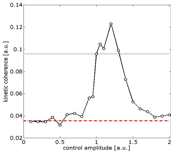
FIG. 7: Kinetic coherence versus \delta for the approximate control term given by Eq. (18). The red dash-dotted line indicates the kinetic coherence value for the non-controlled case and the dotted line the kinetic coherence value for the approximate control term given by Eq. (16). The overlap parameter is s = 1.27 .
