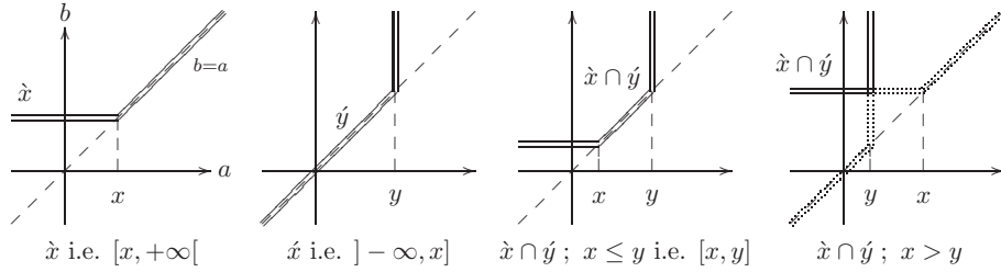
Figure 6: Interval models
