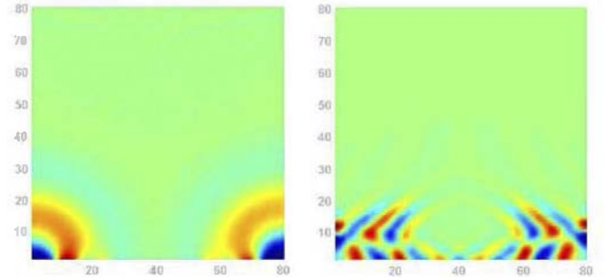
Figure 2: Pressure fields inside the cavity for sub- and super critical waves, finite difference model.
