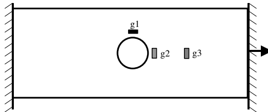
Fig. 2. Traction test on a perforated plate made of [45]_4 woven ply laminate.
