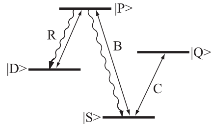
FIG. 1: N Level scheme: The states |D\rangle , |P\rangle , |S\rangle form a \Lambda -configuration; additionally, state |S\rangle couples weakly to the metastable state |Q\rangle . The solid lines and letters R, B, C indicate the laser couplings, the wavy lines the radiative decay channels. Parameters and possible atomic species are discussed in the text.
