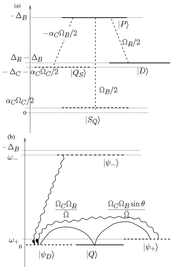
FIG. 2: Dressed states picture for (a) the three-photon resonance case and (b) the two-plus-one-photon resonance case. See text for parameters and definitions.
