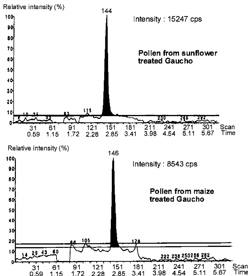
Figure 3. Typical chromatograms of pollen (detection at m/z = 209 ). (A) Pollen from sunflower treated with the Gaucho seed dressing (1.7 \mu\text{g/kg} ). (B) Pollen from maize treated with the Gaucho seed dressing (1.4 \mu\text{g/kg} ). The relative intensity scale corresponds to 100% of the peak height, whereas the amounts of imidacloprid were deduced from peak integration according to the calibration of each run. Analytical data satisfied the criteria reported in the validation section.
