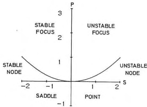
FIGURE 2. The nature of steady states in two-variable systems. The location of a steady state in S-P space with respect to the axes and the parabola S^2 - 4P = 0 indicates the nature of the steady state. S is the sum and P is the product of the roots of the characteristic equation.
