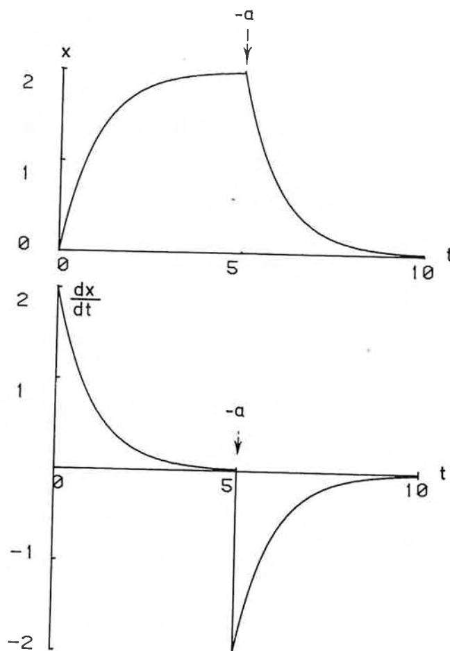
FIGURE 1. The system \frac{dx}{dt} = ka - k_x x . Above: plot of x as a function of time. Initially, x = 0 . At time 0, one switches on x synthesis by adding the precursor a . The arrow indicates that one removes a . Below: plot of \frac{dx}{dt} in the same conditions.
