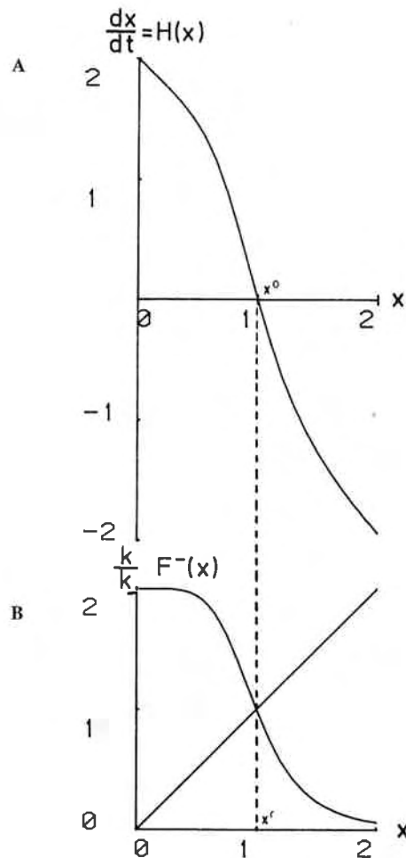
FIGURE 1. One-element negative loop: \frac{dx}{dt} = H(x) = kF^-(x) - k_x x . (A) The time derivative H(x) as a function of x . The intersect of the curve with the x axis is the steady-state value x^0 . In our particular case, H(x) = \frac{2}{1+x^5} - x . (B) The steady-state equation \frac{dx}{dt} = 0 or kF^-(x) - k_x x = 0 can be written x = \frac{k}{k_x} F^-(x) , or x = G^-(x) . If, instead of plotting H(x) as a function of x , one plots G^-(x) , the steady state will be given by the intersect between G^-(x) and the bissectrix. In the particular case given here, the steady-state equation is \frac{2}{1+x^5} - x = 0 , or x = G^-(x) = \frac{2}{1+x^5} . The steady-state value (the solution of the steady-state equation), x^0 = 1 , is readily found by iteration (see Appendix 1).
