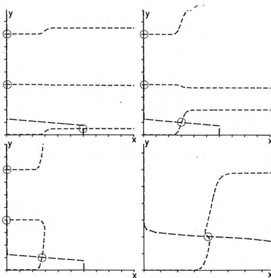
FIGURE 1. The nullclines of Cases 1, 2, and 3 for n = 20 . As usual, long dashes are used for the nullclines dx/dt = 0 and short dashes for dy/dt = 0 .
