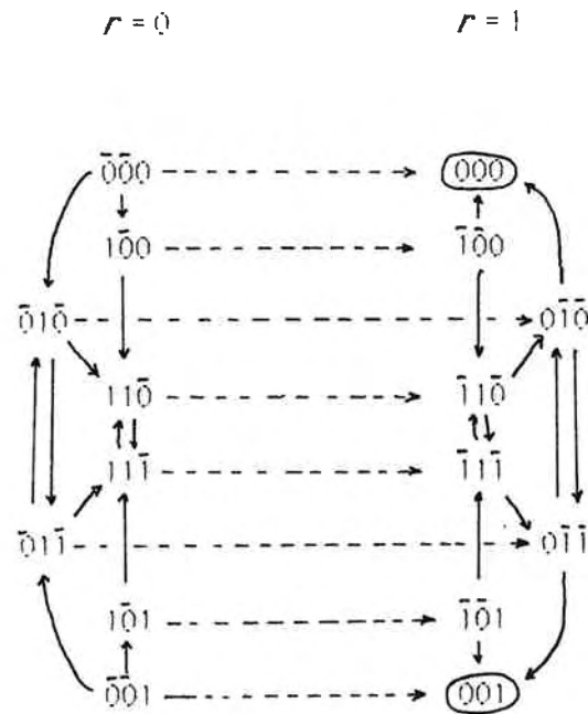
FIGURE 2. Integration pathways of a \lambda_{gal} to the left of a prophage. The variables are listed in the order c , i , l , as in the text.
