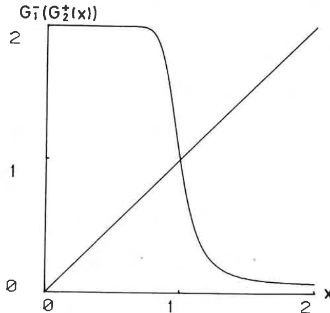
FIGURE 4. The steady-state value x^0 of the system described in Figure 3 can also be found as the intersect of G_1(G_2^*(x)) with the bisectrix.
