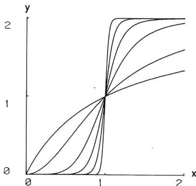
FIGURE 2. Sigmoid functions (more specifically, y = \frac{2x^n}{1+x^n} , with increasing values of the Hill number ( n = 1, 2, 5, 10, 20, \text{ and } 50 ).
