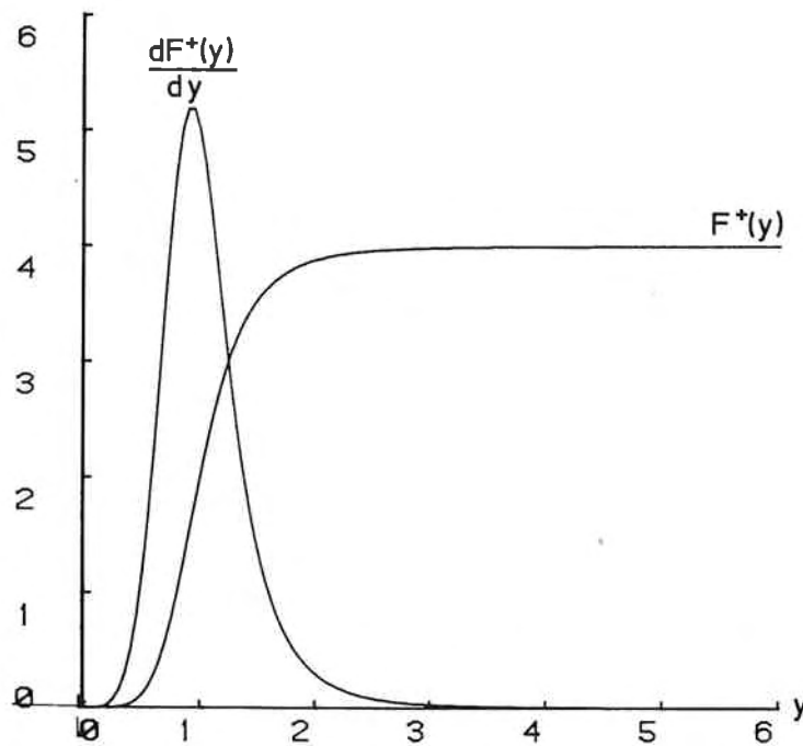
FIGURE 3. The functions dF^+(y)/dy and F^+(y) . The maximum of dF^+(y)/dy corresponds to the inflection point y_i of F^+(y) . The point y_i is less than the threshold value \vartheta_{22} ( \vartheta_{22} = [(n + 1)/n - 1]^{1/n} y_i ), but the steeper the sigmoid (i.e., the higher the Hill exponent n ), the closer the two points will be. It is also clear that the steeper the sigmoid is, the higher and narrower the derivative curve will be.
