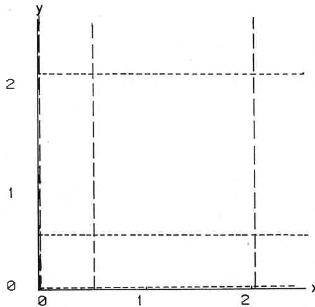
FIGURE 1. Nullclines of the system (1). As usual, the nullcline dx/dt = 0 is in long dashes and dy/dt = 0 is in short dashes. For clarity, nullclines that lie on an axis are shifted slightly.
