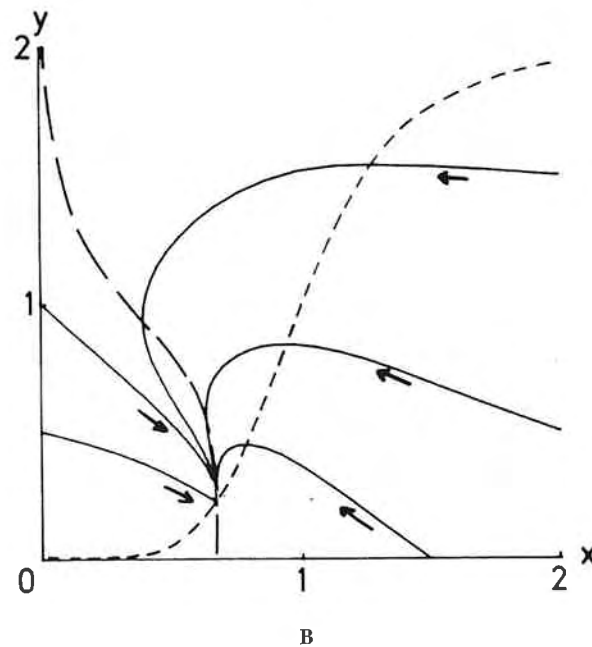
FIGURE 5. Nullclines and trajectories in System 2. (A) Parameter values as in Figure 3 and 4; (B) parameter values as above, except that k_{-1} = 3 instead of 1. The trajectories show and the linear stability analysis (Appendix 3, examples 1 and 2) confirms that in (A) the steady state is a stable focus and in (B) it is a stable node.
