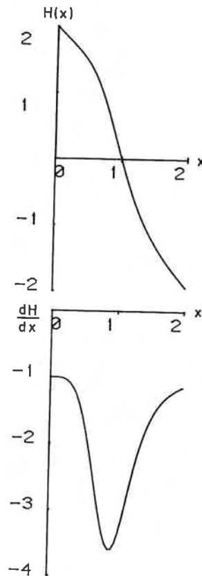
FIGURE 1. Plot of \frac{dx}{dt} , or H(x) , and of \frac{dH}{dx} as functions of x for the one-variable system H(x) = kF^{-1}(x) - kx . Specifically, we take:
