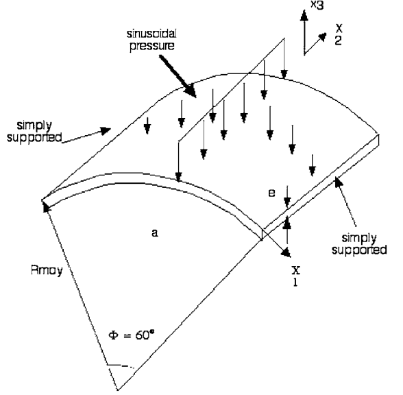
Fig. 1. The Ren laminated cylindrical shell panel.
