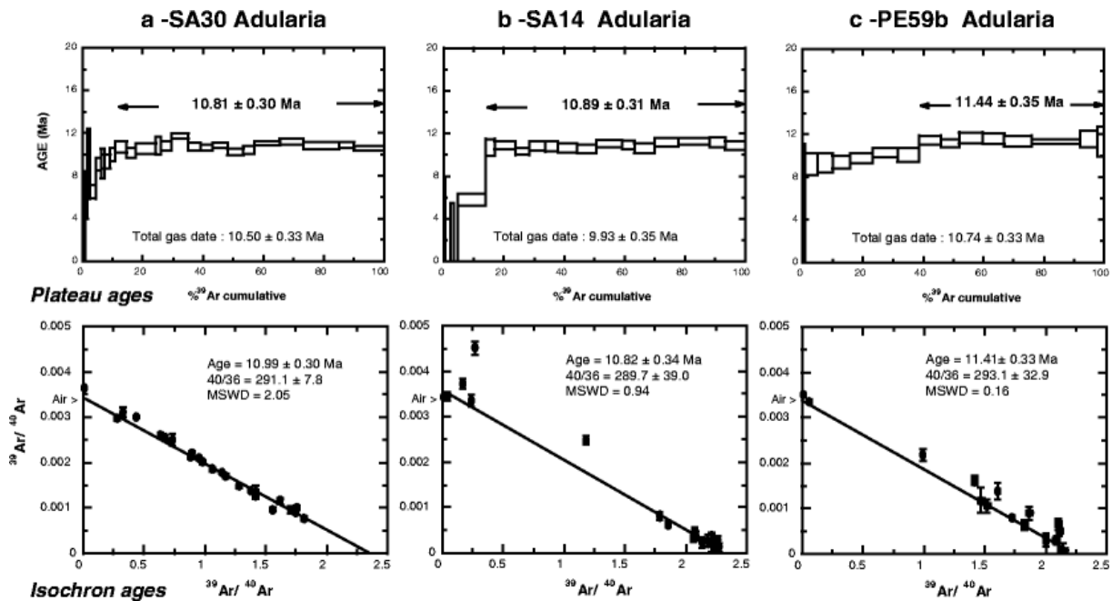
Fig. 15 40 Ar/ 39 Ar results for the three analyzed samples represented by plateau-age spectra and isochron diagrams
