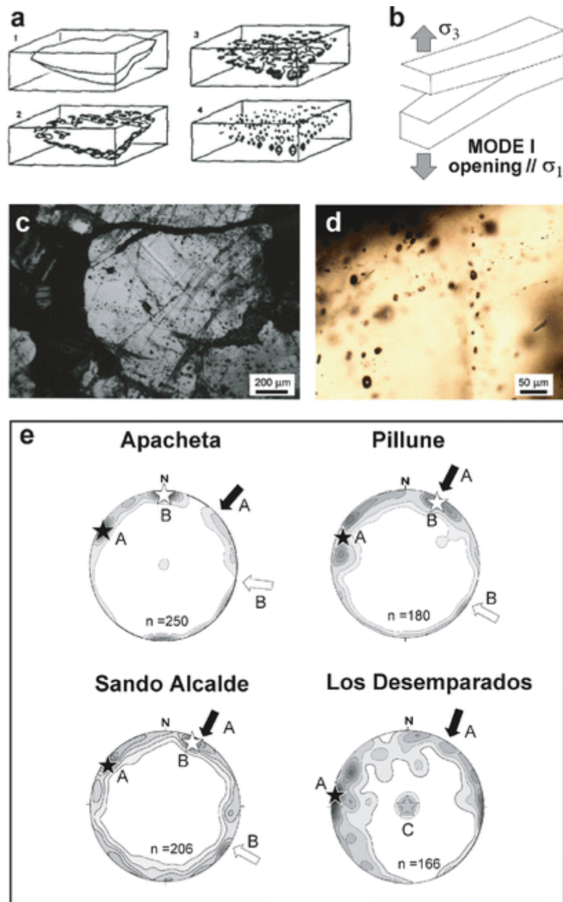
Fig. 13 Fluid inclusion plane (FIP) geometry. a Mode of FIP formation by fracturing and healing (Roedder 1984). b Schematic position of FIP with respect to \sigma_1 and \sigma_3 stress (Atkinson 1987). c and d FIP within magmatic quartz grains. e Stereonet diagrams showing the distribution of FIP within selected samples from the Apacheta, Pillune, Sando Alcalde, and Los Desemparados areas (see text for explanation)
