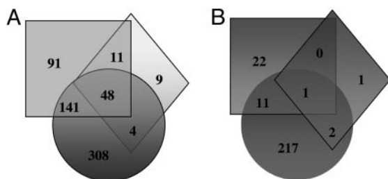
Fig. 2. Number of genes induced (A) or repressed (B) in low Pi. Comparison of short-term (diamonds), medium-term (squares), and long-term (circles) experiments. The whole plant was analyzed to monitor the regulation of Pi-responsive genes during short- and medium-term experiments. Results from leaves and roots analyzed separately were mixed as long term experiment.
