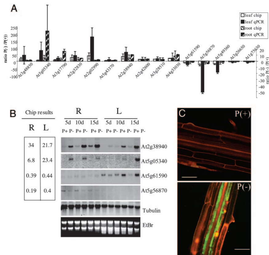
Fig. 3. Validation of ATH1 results. (A) Comparison of chip results and q-PCR. P(-)/P(+) ratio in leaves and roots for some selected genes are shown. Two different scales were used for the genes that were up- or down-regulated. Q-PCR and ATH1 results are means and SD of three assays performed on triplicates. (B) Northern blot analysis and chip results [ratio P(-)/P(+)] of Pi-responsive genes in leaves (L) and roots (R). Plants were harvested after 5, 10, and 15 days of transfer in low [P(-)] or high Pi [P(+)], and 10 \mu g of total RNA, isolated from the whole plant, was hybridized with ^{32} P-labeled cDNA fragments of the genes. Equivalence of RNA loading in all of the lanes is shown by ^{32} P-labeled tubulin hybridization and ethidium bromide-stained rRNA (Lower). (C) Expression of GFP fused to At5GK2 (At3g08720) promoter in the stele and emerging lateral roots of transgenic plants grown under high [P(+)] and low Pi [P(-)]. (Scale bar, 50 \mu m.)
