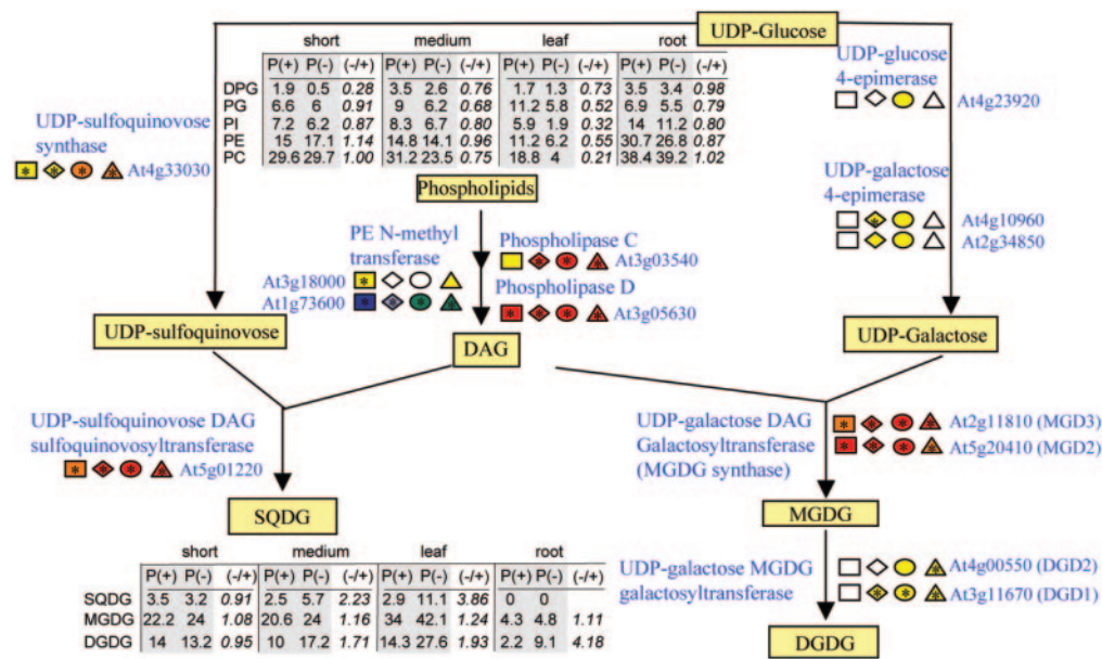
Fig. 4. Transcriptional regulation in pathway of glycosylglyceride biosynthesis in short-term (squares), medium-term (diamonds), and long-term [leaves (circles) and roots (triangles) analyzed separately] experiments. Fold change: red, >10; orange, 4–10; yellow, 2–4; white, 0.5–2; green, 0.25–0.5; pale blue, 0.1–0.25; dark blue, <0.1. *, Significant, one-way ANOVA, P = 0.05 . (Insets) Metabolite quantification [% of total lipids in P(+)] and P(-) and ratio P(-)/P(+)] in short-, medium- and long- (leaf, root) term treatments. DPG, diphosphatidylglycerol; PG, phosphatidylglycerol; PI, phosphatidylinositol; PE, phosphatidylethanolamine; PC, phosphatidylcholine; SQDG, sulfoquinovosyl-diacylglycerol; MGDG, galactosyl-1,2-diacylglycerol; DGDG, digalactosyl-diacylglycerol.
