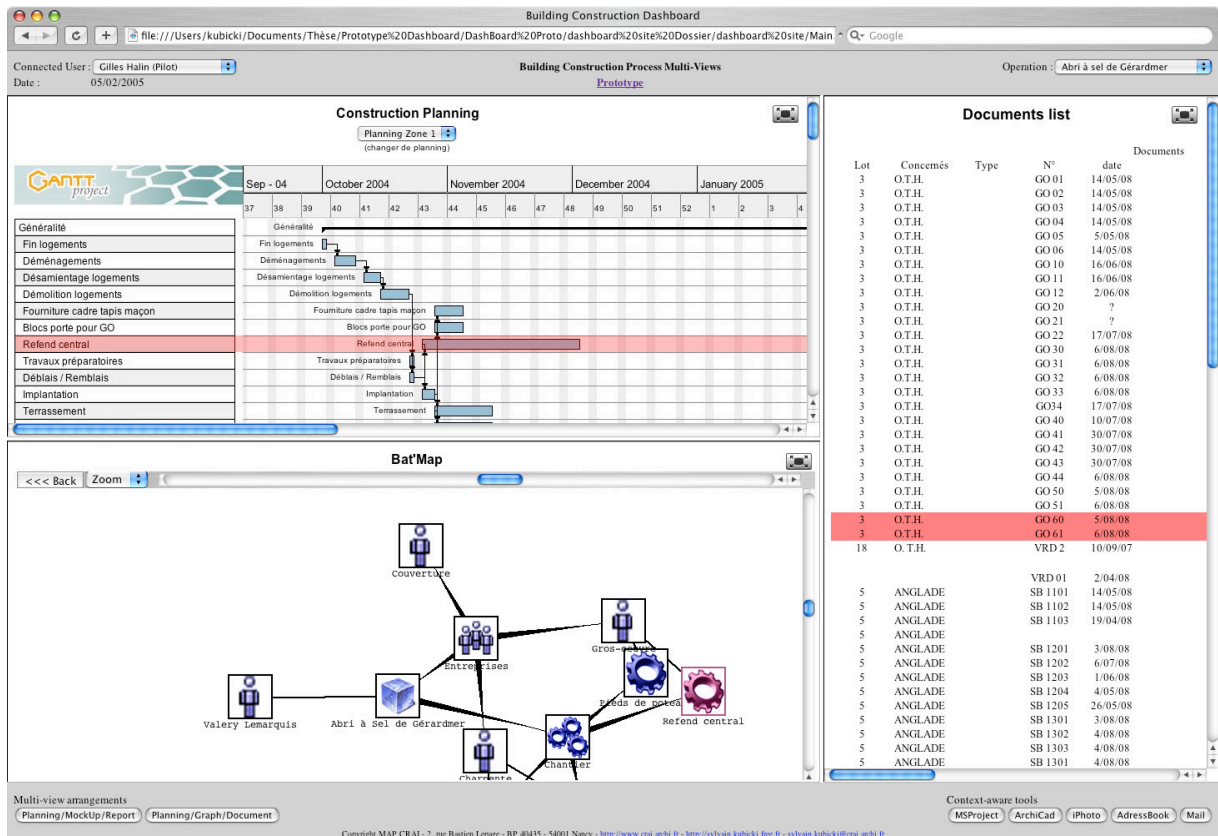
FIG. 8: A hypothesis of the multi-view interface – Coordinator view
