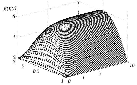
Fig. 2. Evolution of g(t, y) for c = 1 , Re = 1 .
