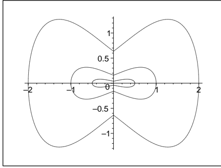
Figure 2: Intersection of different level sets with a vertical plane.
