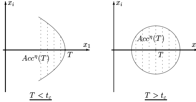
Figure 1: Hyperbolic case
