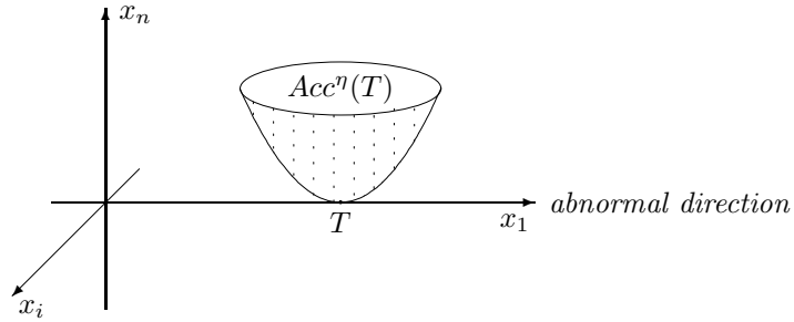
FIGURE 1. Shape of \text{Acc}^\eta(T) , T small
