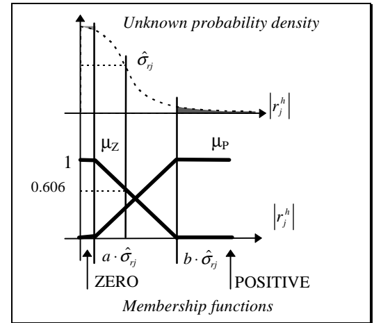
Figure 2: Residual fuzzification.
