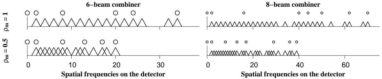
Figure 5. Results of plane optimization for a 6-beam (left) and 8-beam (right) combiner. The output pupil configuration and the Fourier plane are represented at the same scale (autocorrelation relation). The pupil positions are computed for a Compression Factor of \rho = 1 (top) and \rho = 0.5 (bottom). The minimum distance between the pupils is set to twice the pupils width ( N_{fri} = 2 ). The frequency range is reduced by a factor 0.58 and 0.55 in the 6- and 8-beam case respectively.
